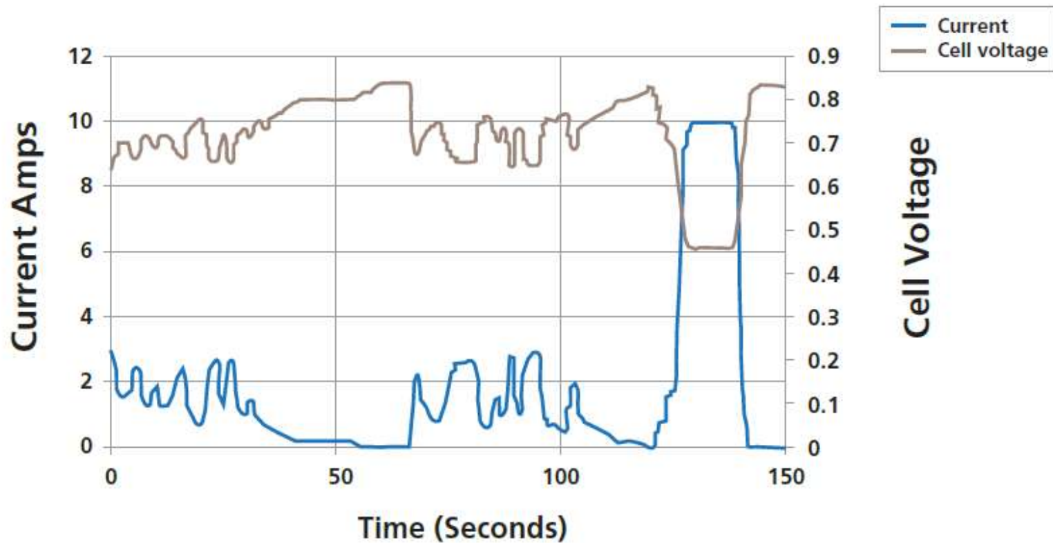
"Instant" Response of FlowCath® Technology
